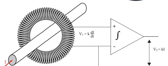
Rogowski coil
